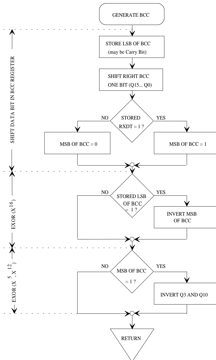
Figure 13: Subroutine 'Generate Block Check Character'
