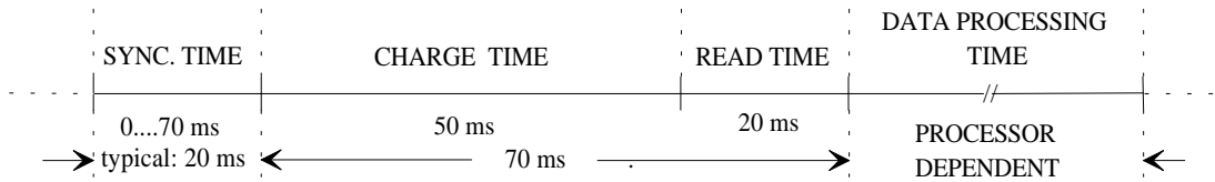
Figure 22: Readout Cycle of a TIRIS Reading/Writing Unit
