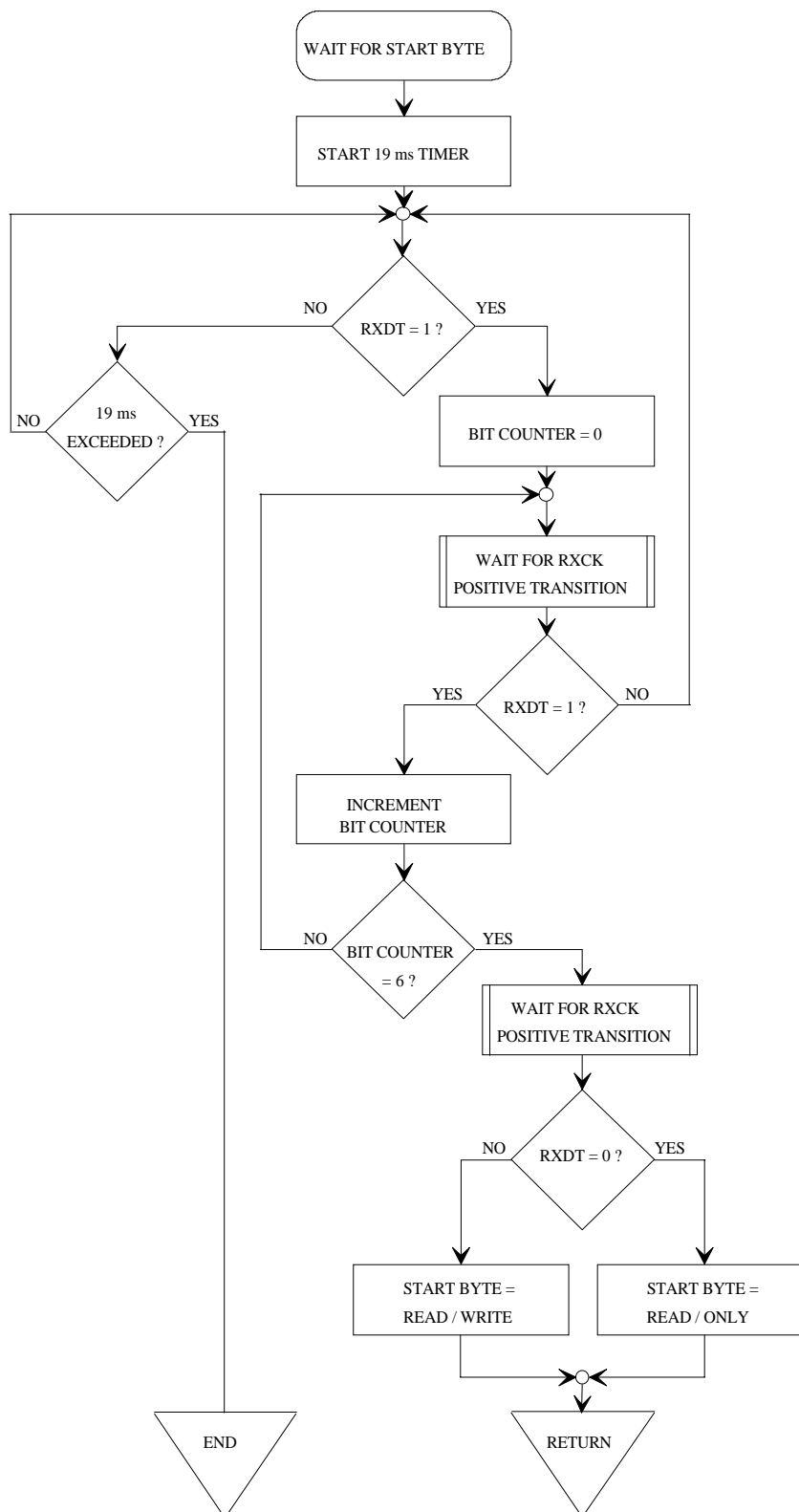
Figure 9: Wait for Start Byte
