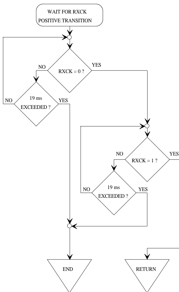
Figure 12: Subroutine 'Wait for RXCK Positive Transition'
