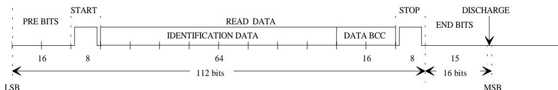
Figure 3: 64-bit Read Only Transponder Read Data Format
