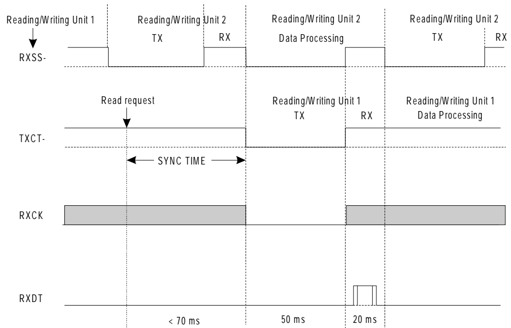
Figure 25: Units 1 & 2 Transmit Simultaneously
