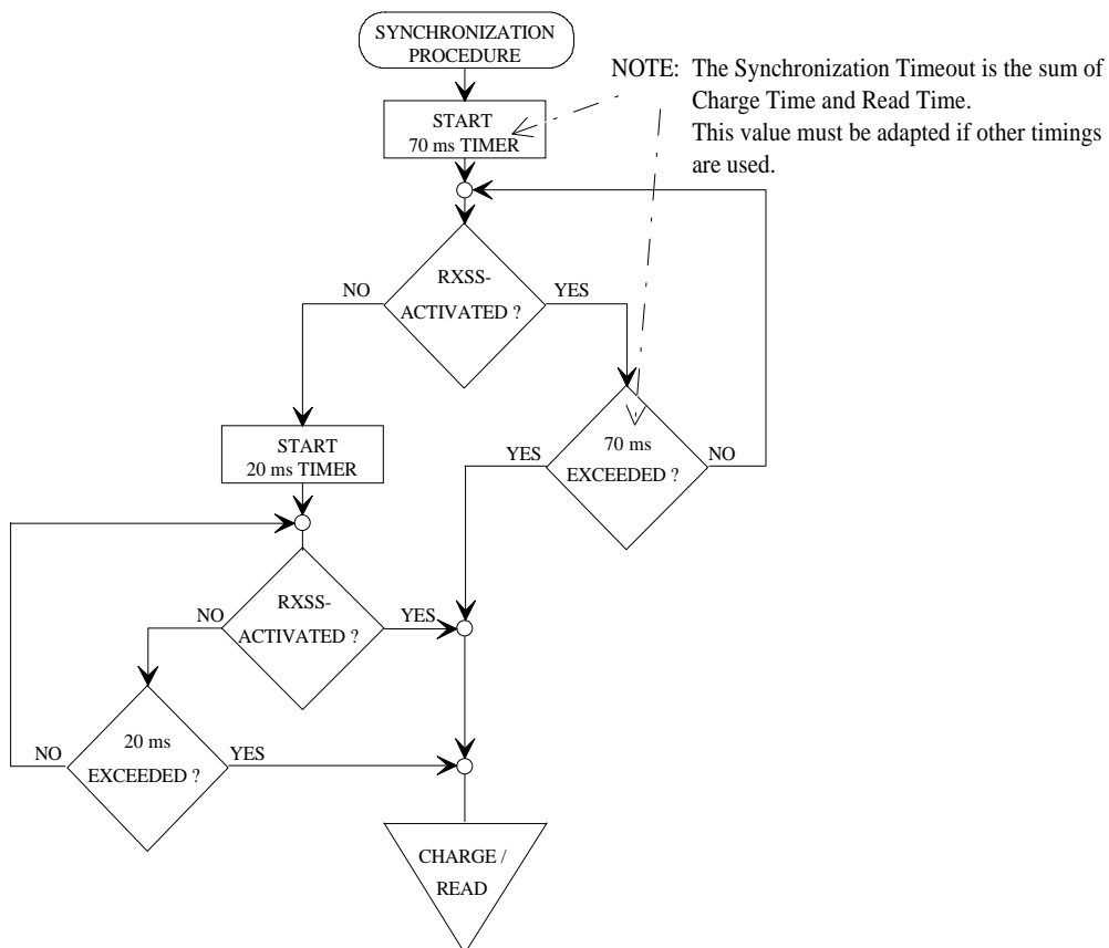
Figure 23: Synchronization Procedure Flowchart
