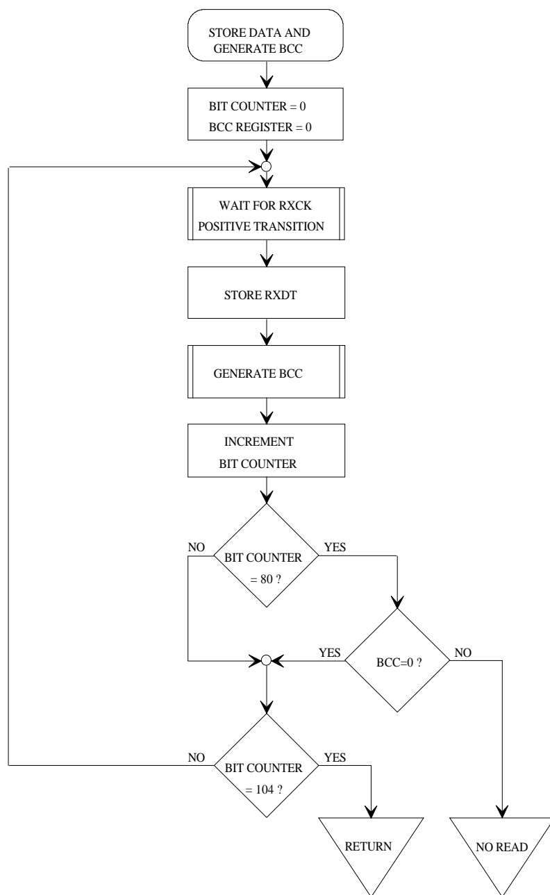
Figure 10: Store Data and Generate Block Check Character
