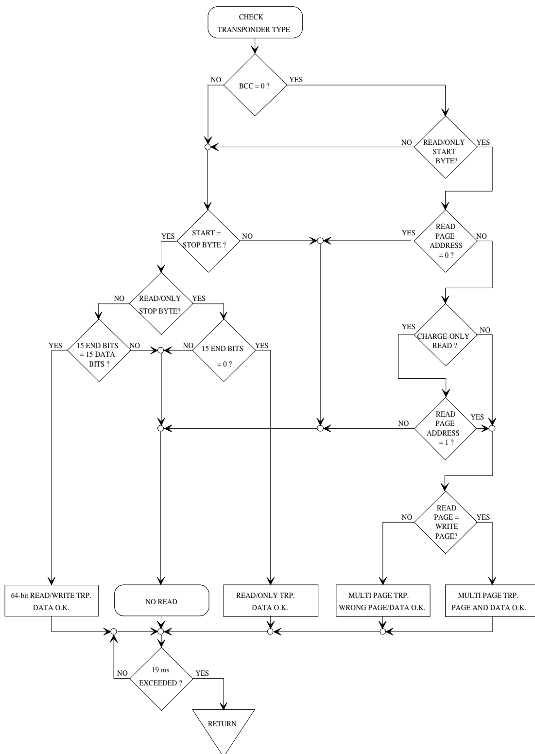
Figure 11: Check Transponder Type
