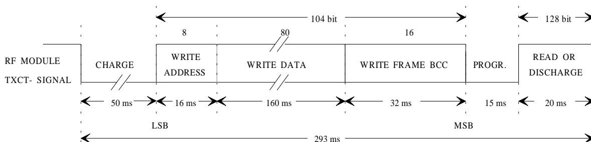
Figure 18: Selective Program Page Function Data Format
