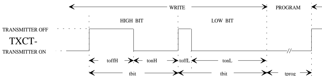
Figure 14: The Write and Program Function
