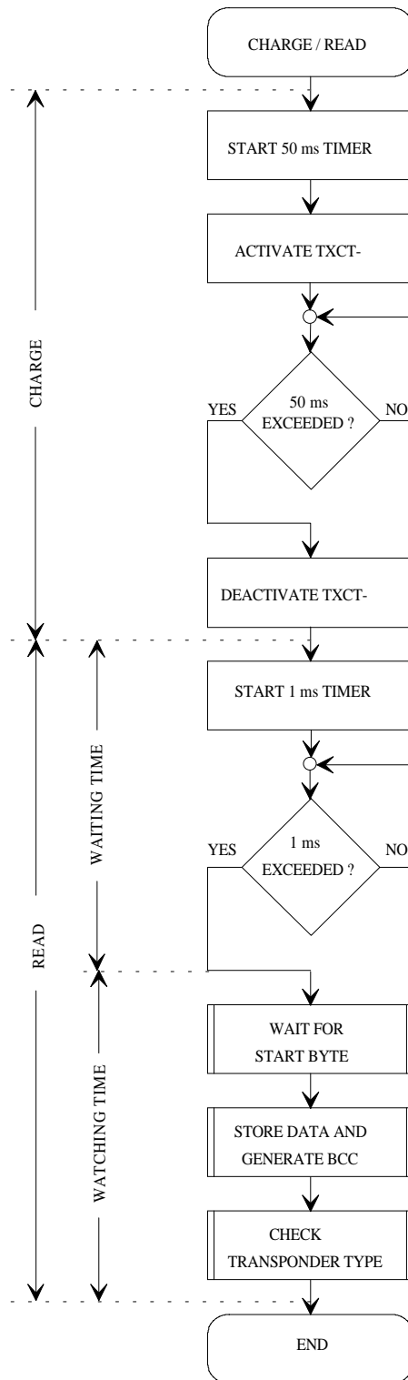
Figure 8: Sequence Control Software Overview
