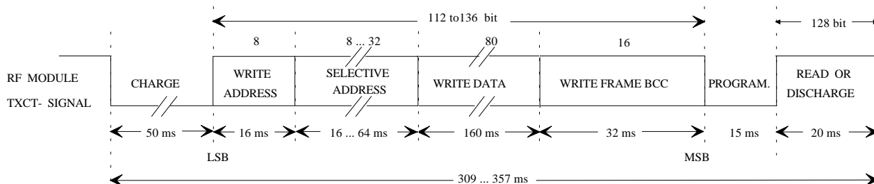
Figure 18: Selective Program Page Function Data Format
