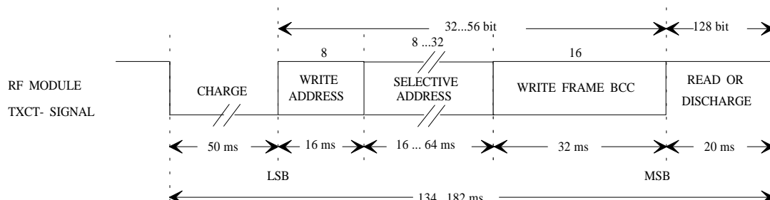
Figure 21: Selective Read Function Data Format
