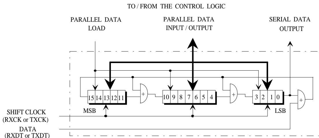
Figure 7: Cyclic Redundancy Check Generator Block schematic
