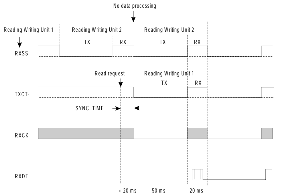
Figure 25: Units 1 & 2 Transmit Simultaneously
