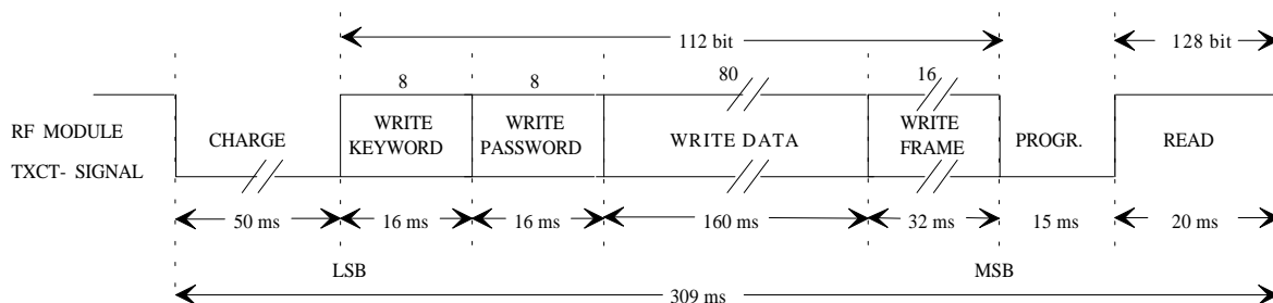
Figure 15: 64-bit Read/Write Transponder Programming Data Format
