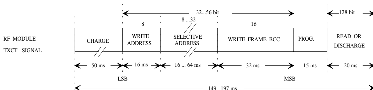
Figure 20: Selective Lock Page Function Data Format
