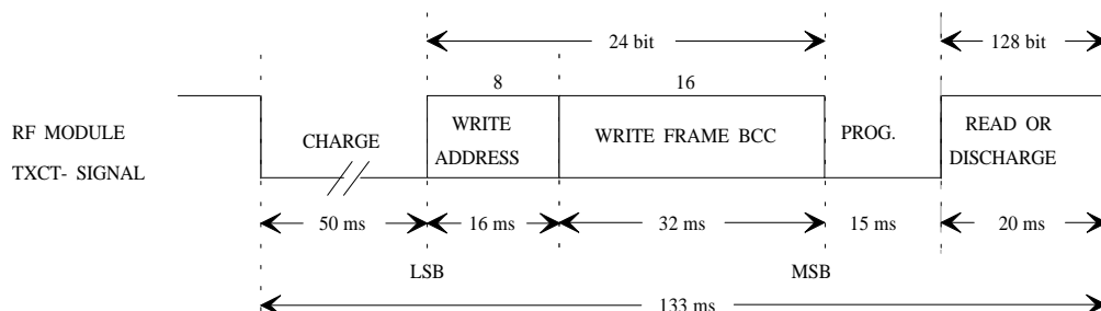
Figure 20: Selective Lock Page Function Data Format
