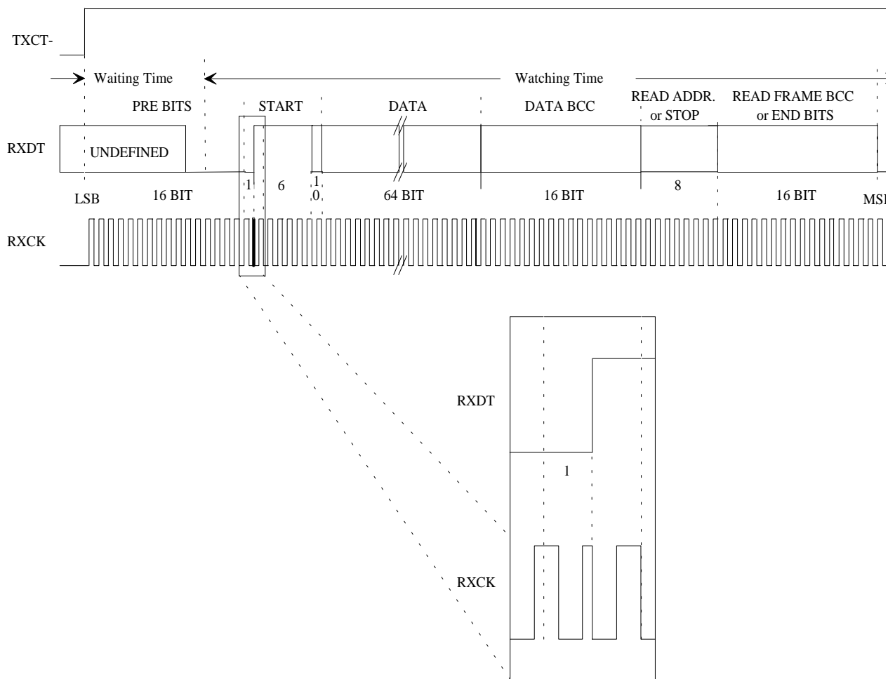
Figure 6: Data Format at the Receiver Outputs
