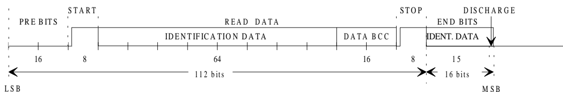
Figure 4: 64-bit Read/Write Transponder Read Data Format
