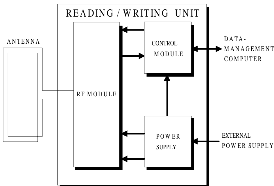
Figure 1: Block Schematic of a Reading/Writing Unit
