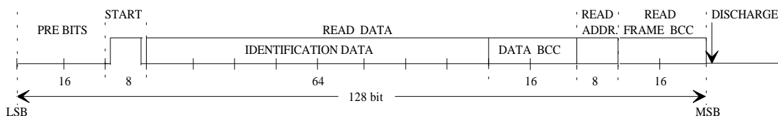
Figure 5: Multipage Read/Write Transponder Read Data Format
