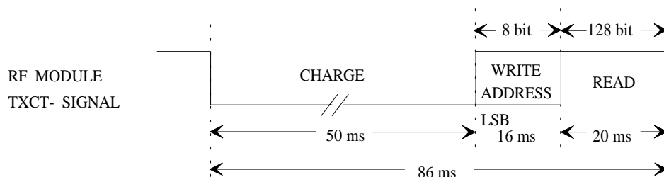
Figure 16: Multipage R/W Transponder General Read Function
